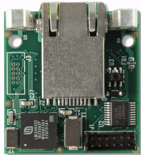
Figure 1. Serial-to-Ethernet Module
